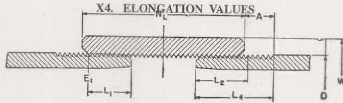
FIG. X3.2 Dimensions of Hand Tight Assembly for Use with Table X3.2
