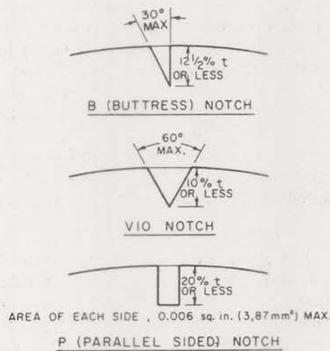
FIG. 1 Calibration Standards
